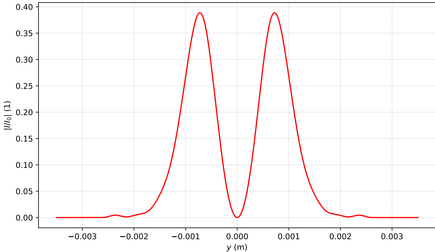
Intensity profile I(x=0, y, z=2.707)/I_0 , \text{Pin}=3.0\text{Pcr} , artificial time
